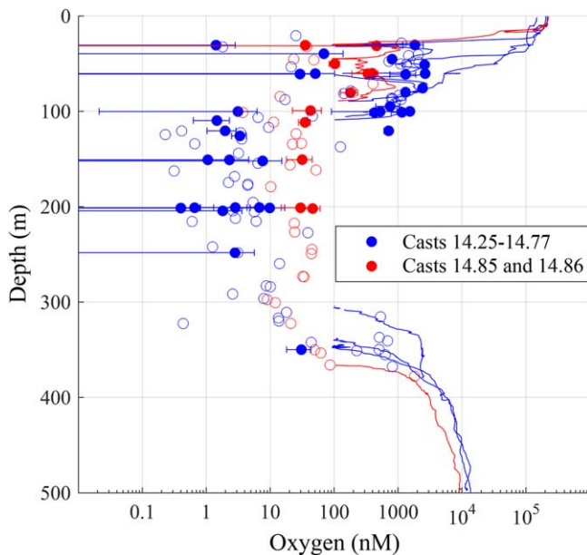
Fig. 1. Oxygen measured by Thamdrup et al. (2012) with the Switchable Trace amount OXYgen (STOX) sensor (circles) and a STOX-calibrated conventional oxygen sensor (lines) in the eastern South Pacific ocean along the west coast of South America. As in Thamdrup et al. (2012), locations with multiple measurements (solid circles) include error bars (standard deviations), and locations with one measurement (open circles) have a detection limit of 10 nM. Error bars that intersect with the y-axis signify error to or below zero. Oxygen was consistently below 10 nM at the core of the anoxic zone at five sites, with nine total casts (blue), and varied from 10 nM to 50 nM at one site, with two casts (red).
