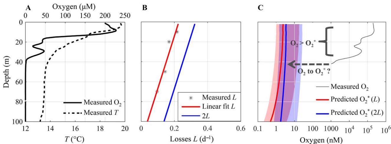
Fig. 3. Predicted O_2^* from measured vertical distributions of (A) temperature, oxygen, and (B) the specific grazing rate on bacteria by heterotrophic nanoflagellates at a coastal upwelling site off Iquique, Chile (20.06°S, 70.19°W; Cuevas and Morales 2006). O_2^* is calculated with and without an additional loss rate of 0.1 \text{ d}^{-1} . For both estimates, (C) calculations reflect the average coastal growth efficiency of 0.19 (lines) with uncertainty due to its standard deviation of 0.16 (shaded regions). Measured oxygen concentrations (A and C) are omitted below the detection limit of 1 \mu\text{M} .
