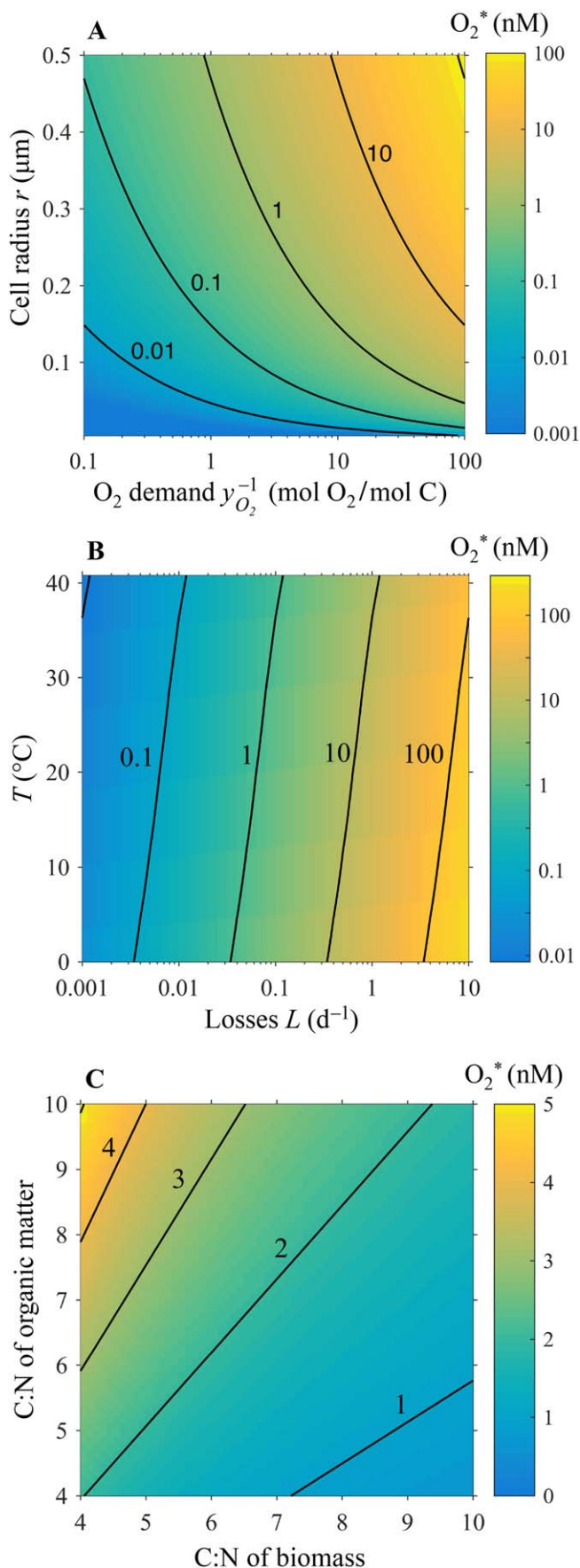
Fig. 2. O_2^* as a function of (A) cell radius r and oxygen demand y_{O_2}^{-1} , (B) losses L and temperature T (via D , the diffusion coefficient for oxygen in seawater), and (C) the C : N stoichiometry of organic matter substrate and biomass composition (Supporting Information Appendix A). Unless varying, parameters are set as best estimates for marine oxygen minimum zones: L = 0.1 \text{ d}^{-1} , T = 12^\circ\text{C} , r = 0.25 \mu\text{m} , and y_{O_2}^{-1} = 7 \text{ mol } O_2 / \text{mol C} .
