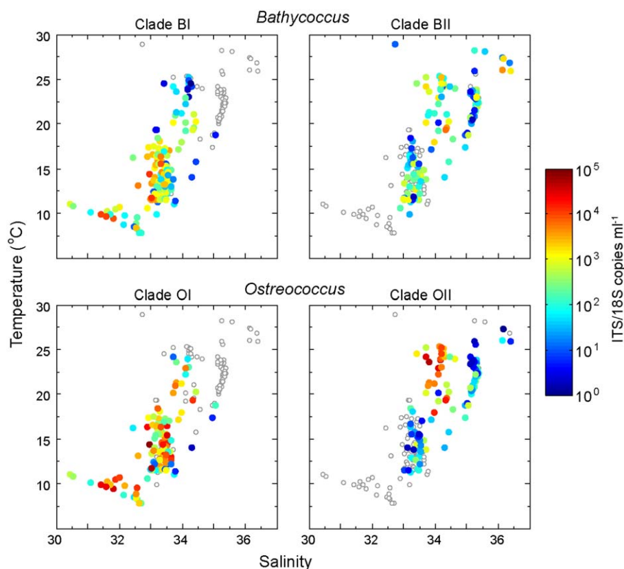
Fig. 6. Patterns across multiple oceanic regions establish clade relationships with temperature and salinity. Bathycoccus clades BI and BII were detected in 152 and 153 samples, respectively, and Ostreococcus clades OI and OII in 131 and 124 samples, respectively. At least one of these taxa was present in 241 of the 259 total samples. Open circles indicate where clade was not detected by qPCR.
