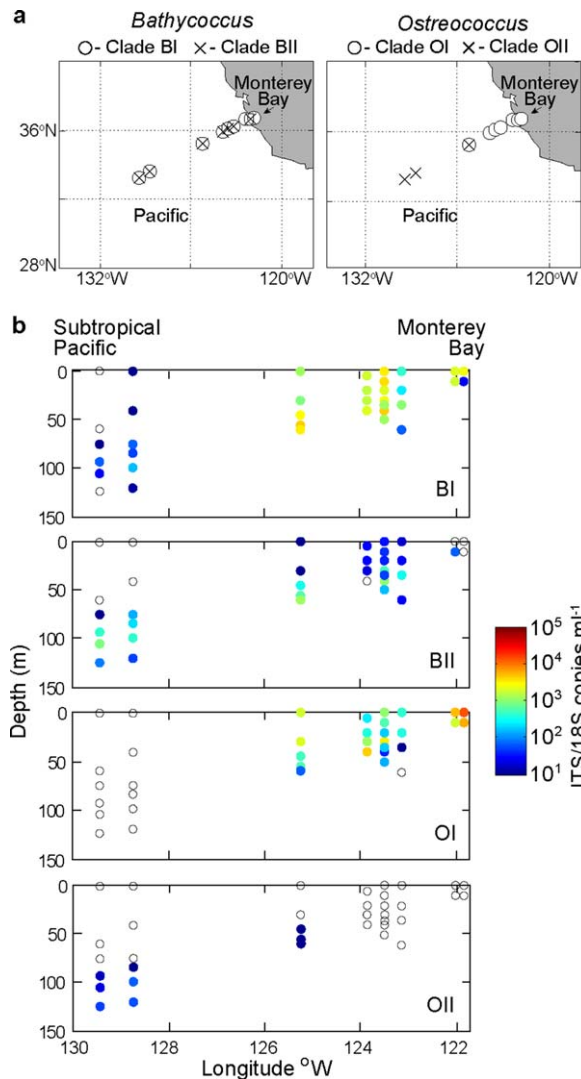
Fig. 5. Abundance of Bathycoccus and Ostreococcus clades along Line-67 in the eastern North Pacific.
