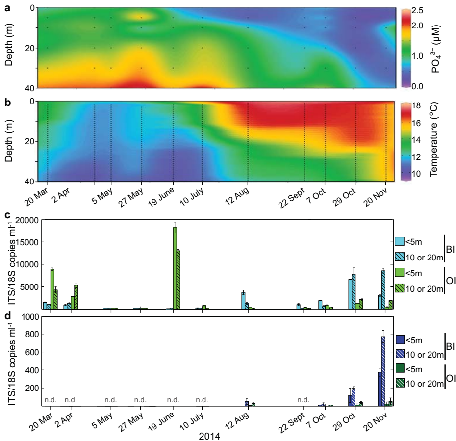
Fig. 3. Dynamics of Ostreococcus and Bathycoccus clades in Monterey Bay, California. Samples were collected at MBTS Station M1 (Pennington and Chavez, 2000). A. Contour plot of \text{PO}_4^{3-} over the study period. Black dots represent CTD data point locations used for extrapolation. B. Contour plot of temperature. C. qPCR abundance of Bathycoccus clade BI and Ostreococcus clade OI at the surface (<5 m) and deeper in the water column (10 m or 20 m) representing the subsurface chlorophyll max, if present, or the base of the wind-mixed surface layer. D. Bathycoccus clade BII and Ostreococcus clade OII qPCR abundances over the study period. Like BII, OII was also found where temperatures were higher ( 15.8^\circ\text{C} \pm 1.1^\circ\text{C} ) and concentrations of \text{NH}_4^+ ( 0.07 \pm 0.07 \mu\text{M} ) and \text{NO}_3^- ( 1.20 \pm 2.31 \mu\text{M} ) as well as N:P ratios ( 1.30 \pm 1.92 ) were lower than samples where not detected. Note the different Y-axis scales in panel C and D. n.d., not detected by qPCR.
