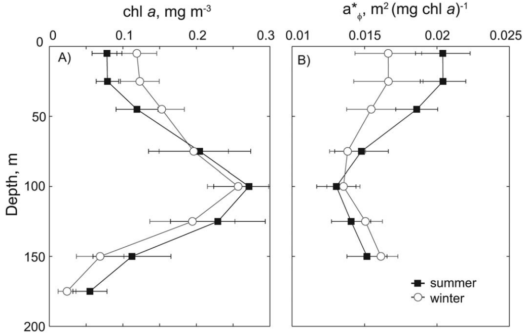
Fig. 4. Depth distribution (mean \pm SD) of chl a concentrations and chl-specific absorption derived from QFT (open circles = winter and closed squares = summer months).
