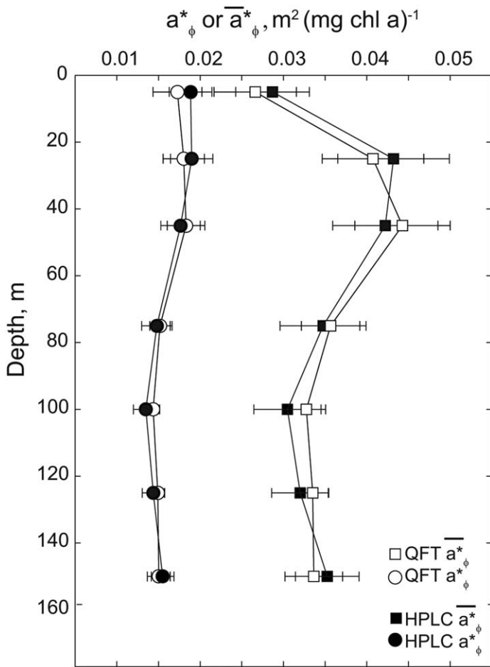
Fig. 7. Depth distribution of total chl-specific absorption unweighted (circles) as well as weighted for the spectral distribution of light (squares). QFT = open symbols, HPLC reconstruction = close symbols.
