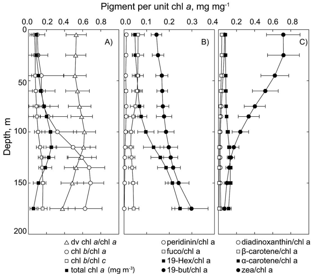
Fig. 5. Depth distribution (mean \pm SD) of HPLC derived chl a concentrations (mv + dv chl a ) and that of accessory pigments concentrations relative to that of chl a . (A) chl pigments (open triangles: [dv chl a /total chl a ], open circles: [chl b /total chl a ], open squares: [chl c /total chl a ], close squares: [total chl a ]). (B) Photosynthetic carotenoids (open circles: [peridinin/total chl a ], open squares: [fuco/total chl a ], close squares: [19-hex/total chl a ], close circles: [19-but/total chl a ]). (C) Photoprotective carotenoids (open circles: [diadinoxanthin/total chl a ], open squares: [ \beta -carotene/total chl a ], close squares: [ \alpha -carotene/total chl a ], close circles: zea/total chl a ).
