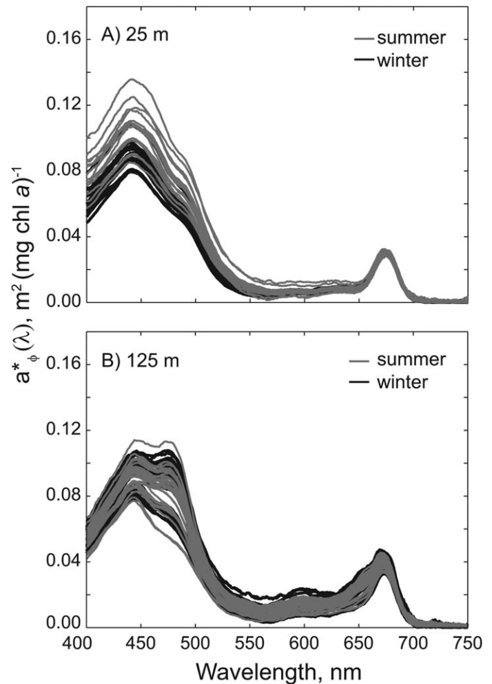
Fig. 3. Ensemble of all summer (grey) and winter (black) QFT derived chl-specific absorption spectra collected at 25 m (upper panel) and 125 m (lower panel).
