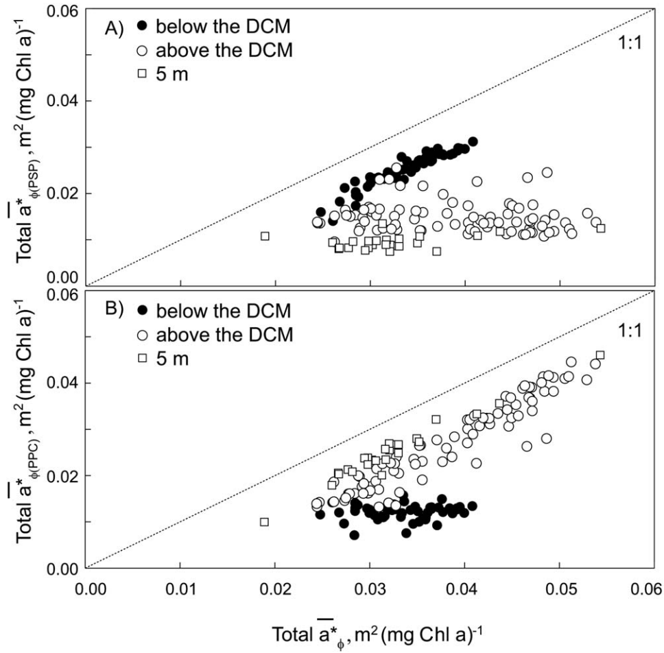
Fig. 8. Chl-specific photosynthetic (upper panel) and photoprotective (lower panel) absorption as a function of total chl-specific absorption. Close symbols = samples collected below the DCM layer; open symbols = sample collected above the DCM layer; open squares = samples collected at 5 m depth.
