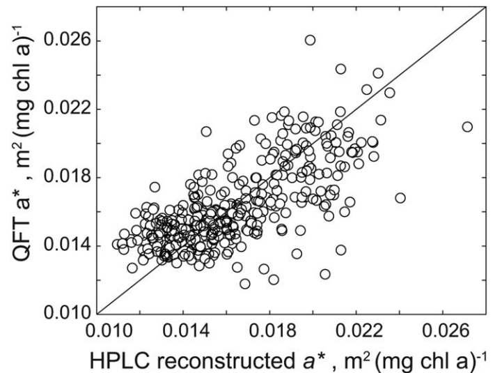
Fig. 2. Relationship between CDOM corrected chl-specific absorption (400–750 nm) derived from QFT and chl-specific absorption from HPLC pigment reconstruction and corrected for packaging effect.
