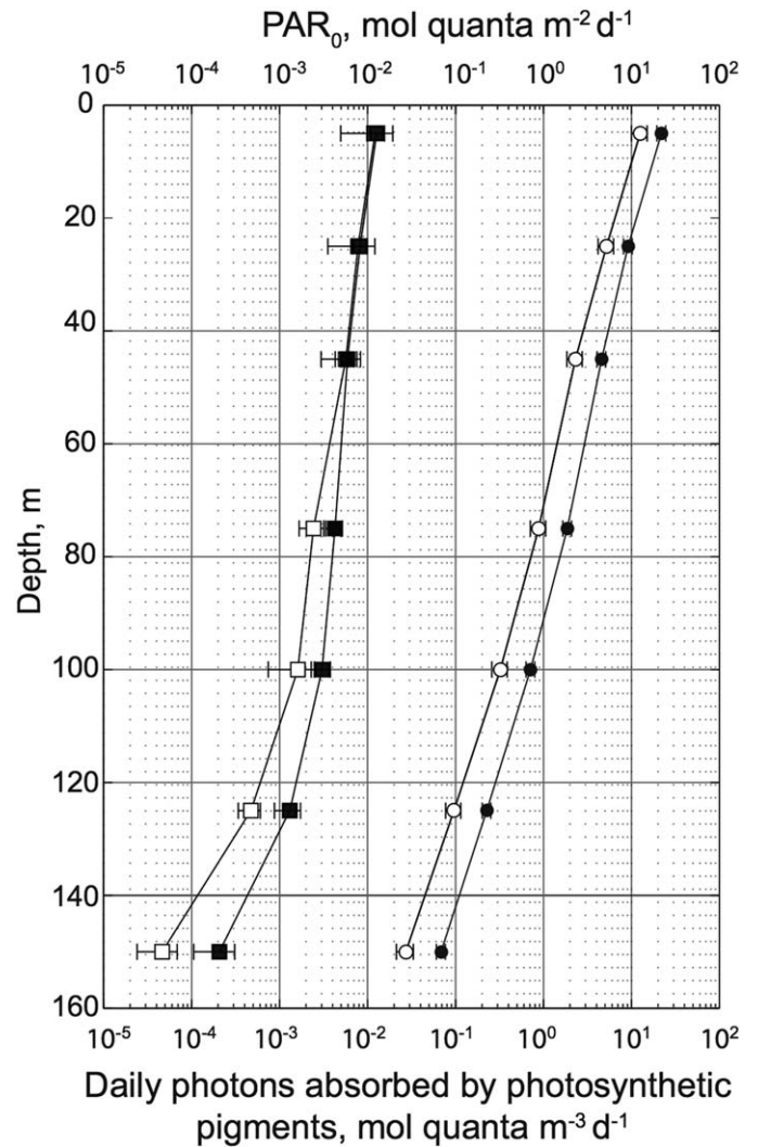
Fig. 9. Seasonal depth distribution of daily PAR_0 (circles) and photon flux absorbed by photosynthetic pigments (squares). Close symbols = summer; open symbols = winter.
