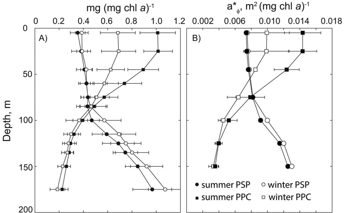
Fig. 6. Relative photosynthetic (circles) and photoprotective (squares) pigments concentration (left panel) and chl-specific absorption (right panel) as a function of depth and season. (Open symbols = winter, close symbols = summer).
