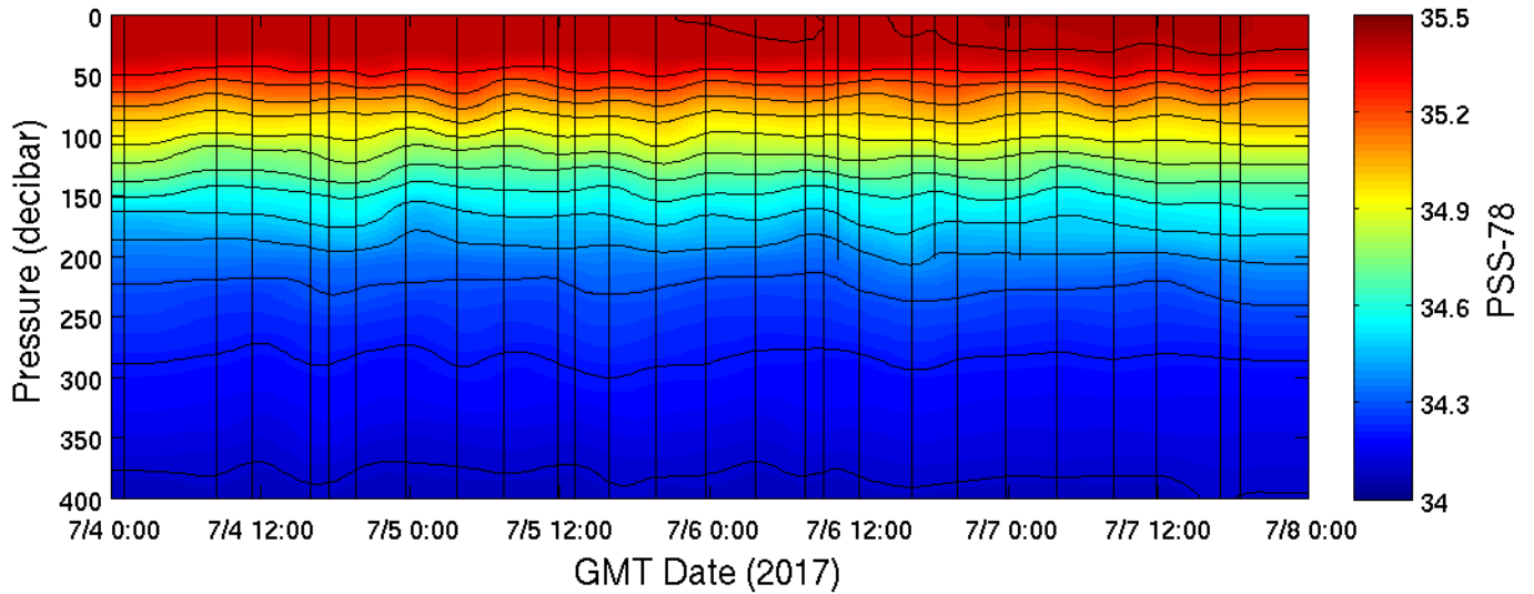
MESO-SCOPE, Cyclone (stn L1), CTD Salinity
