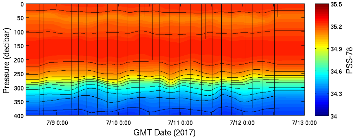
MESO-SCOPE, Anti-cyclone (stn L2), CTD Salinity
