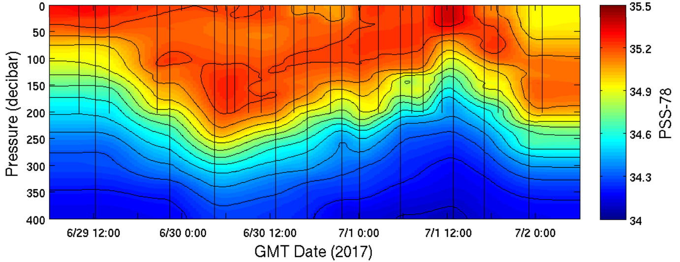
MESO-SCOPE, Dipole transect (stn 4-14), CTD Salinity
