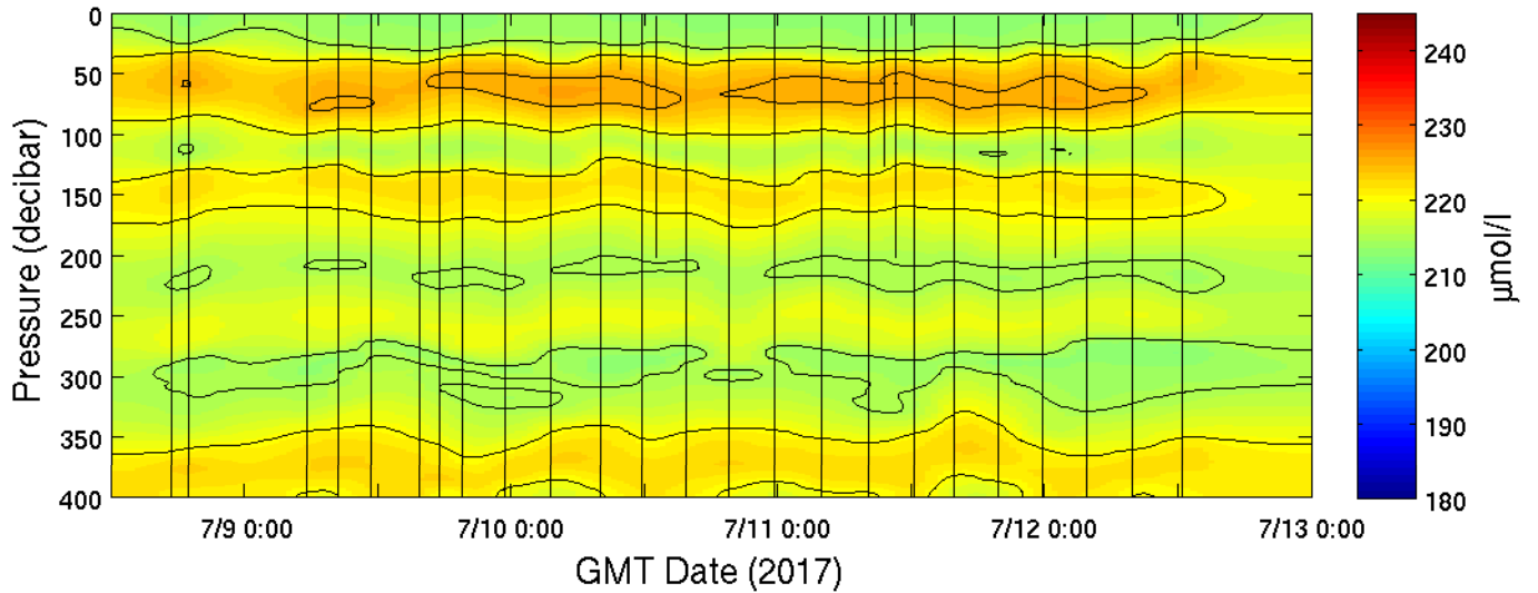
MESO-SCOPE, Anti-cyclone (stn L2), CTD Oxygen
