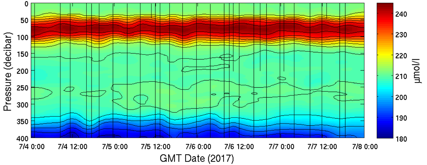
MESO-SCOPE, Cyclone (stn L1), CTD Oxygen
