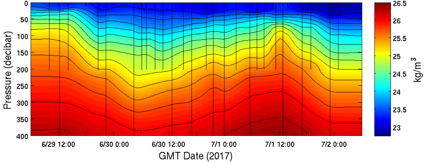
MESO-SCOPE, Cyclone (stn L1), CTD Potential Density
