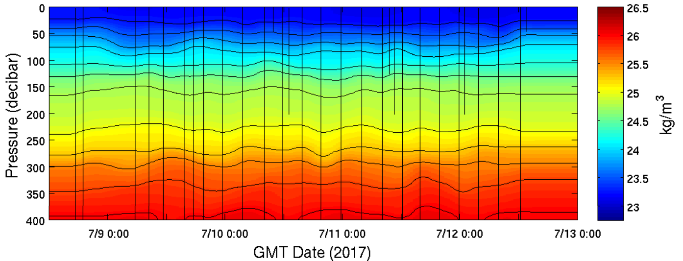
MESO-SCOPE, Anti-cyclone (stn L2), CTD Potential Density
