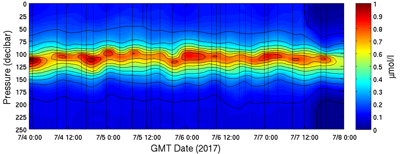
MESO-SCOPE, Anti-cyclone (stn L2), CTD Chloropigment
