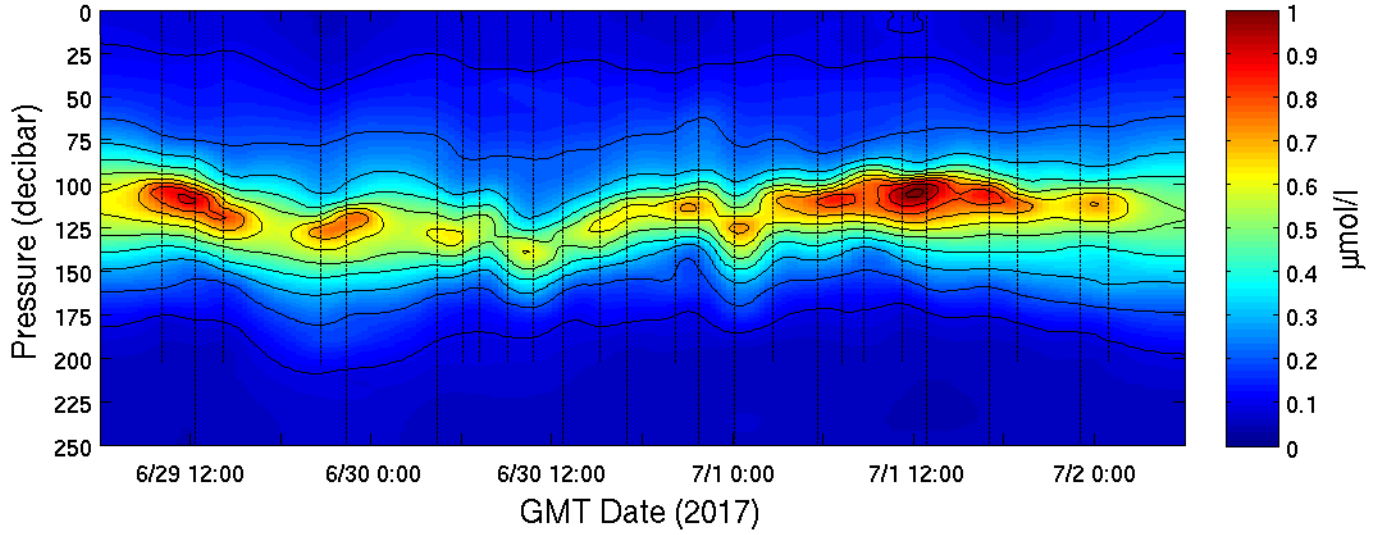
MESO-SCOPE, Cyclone (stn L1), CTD Chloropigment
