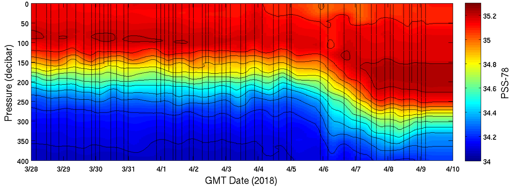
FK180310, Leg-2, CTD Salinity
