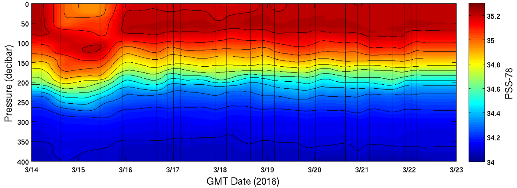
FK180310, Leg-1, CTD Salinity
