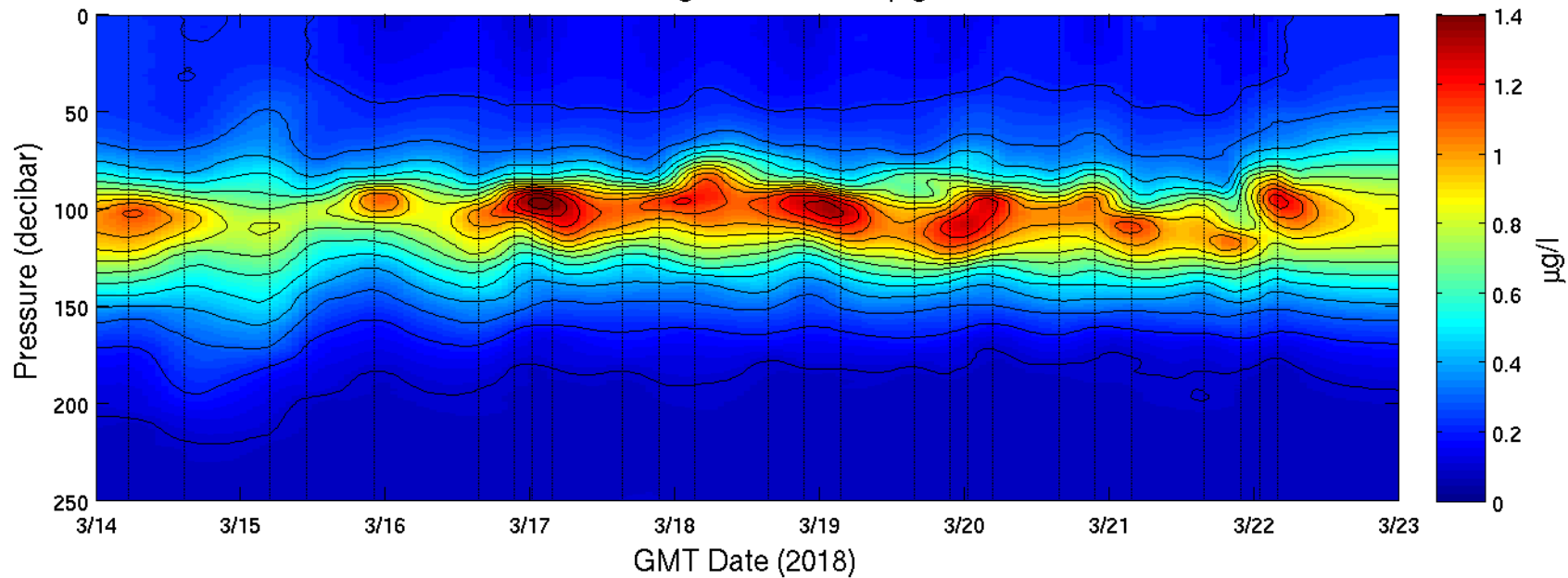
FK180310, Leg-1, CTD Chloropigment
