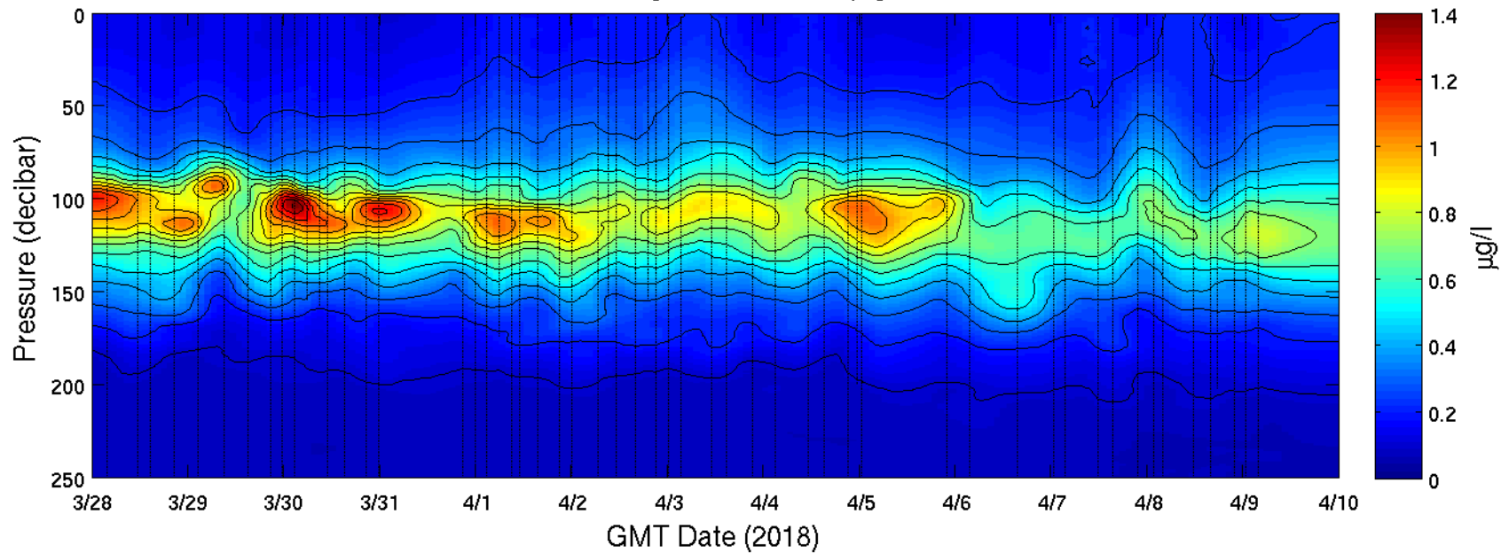
FK180310, Leg-2, CTD Chloropigment
